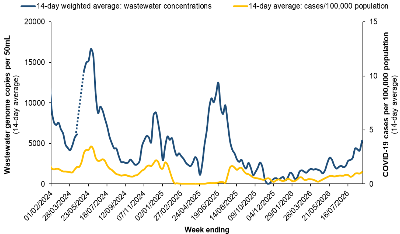
Figure 17. SARS-CoV-2 concentration in wastewater and COVID-19 notification rate, Perth metropolitan area, WA, 2024 to 28 August 2026.
