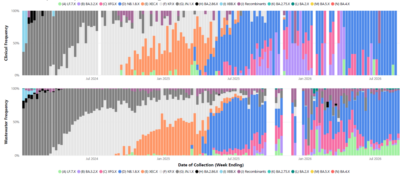
Figure 18. Distribution of SARS-CoV-2 variants in clinical samples (top) and metropolitan wastewater catchments (bottom), 01 Jan 2024 to 30 Aug 2026
